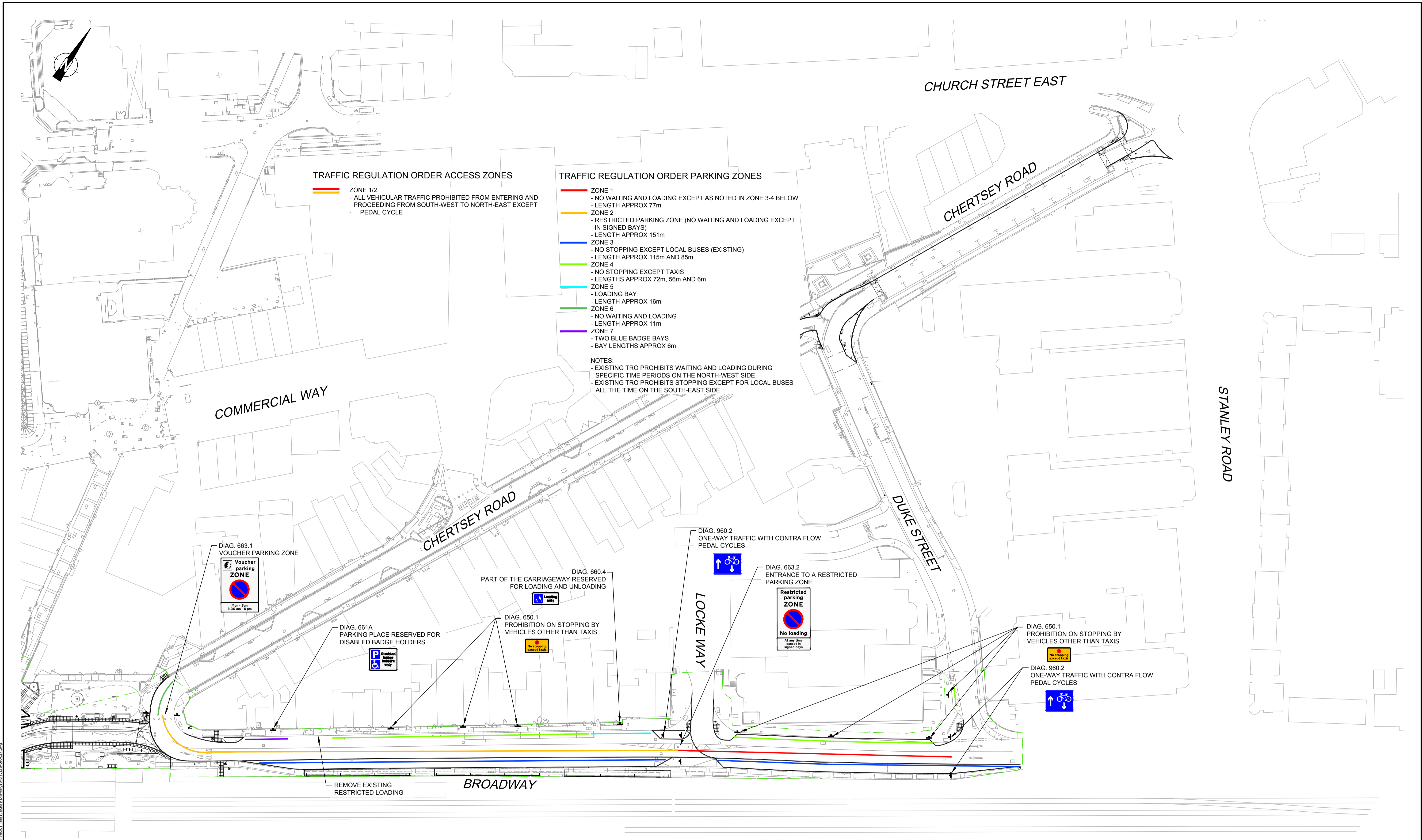
PLAN SCALE 1:500
