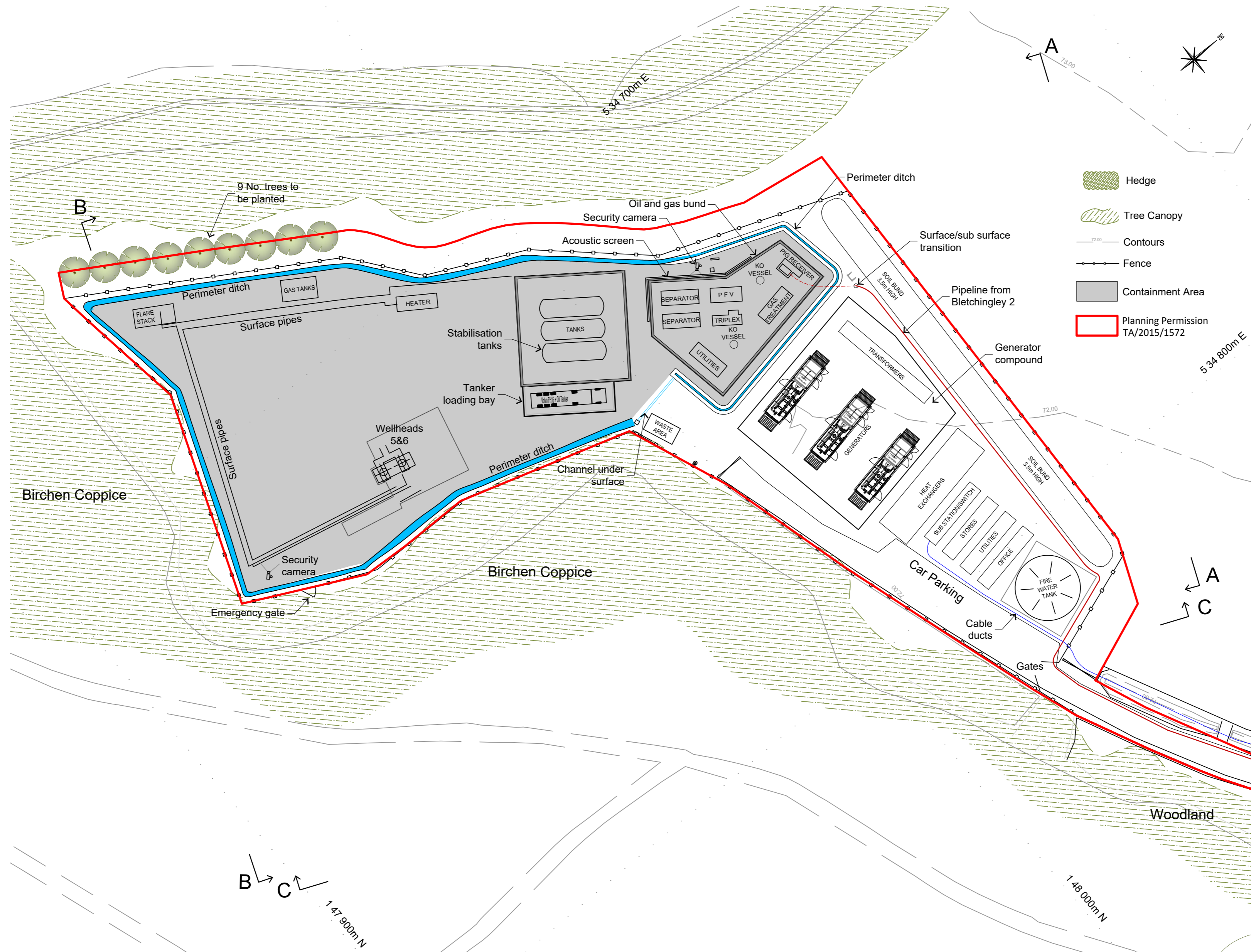
Preliminary Wellsite Layout - Bletchingley Central Scale 1:500
